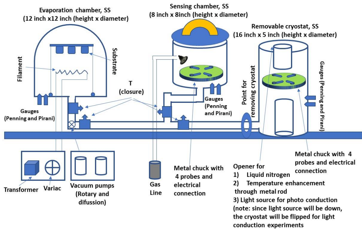
Figure 1: Drawing of the vacuum-based cluster tool for electrical and sensing characterizations and metal contact deposition.
