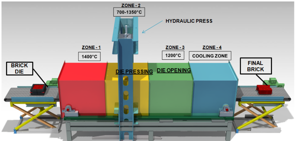
The schematic of semi-automated hot press, which is indent to build to make the joint free gamma and neutron shielding blocks.
